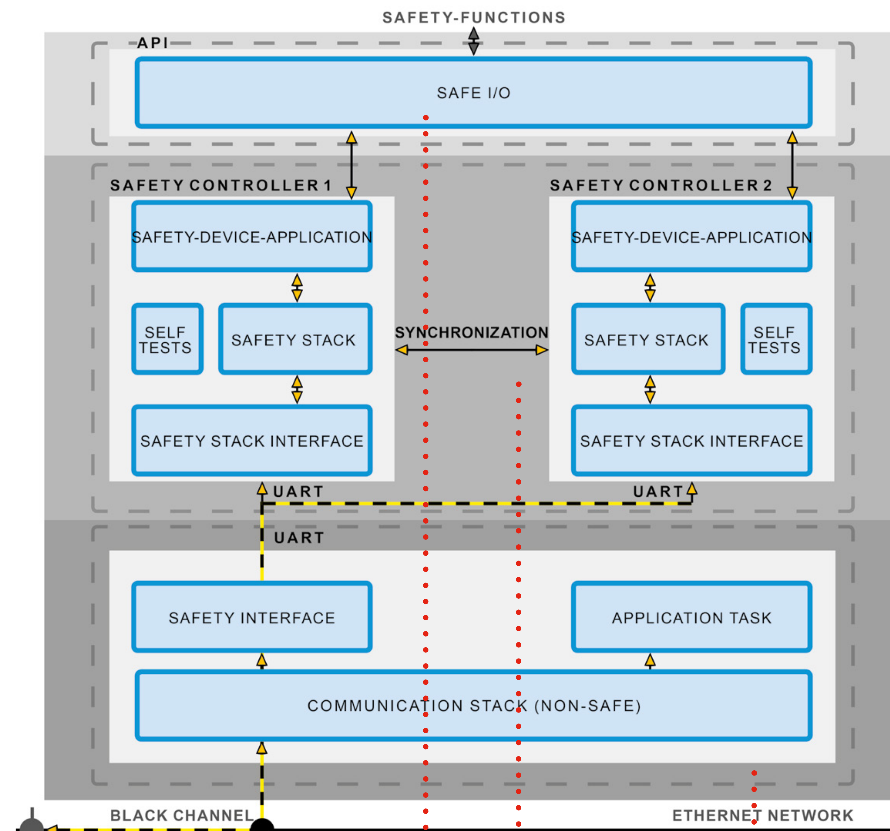
Software architecture
